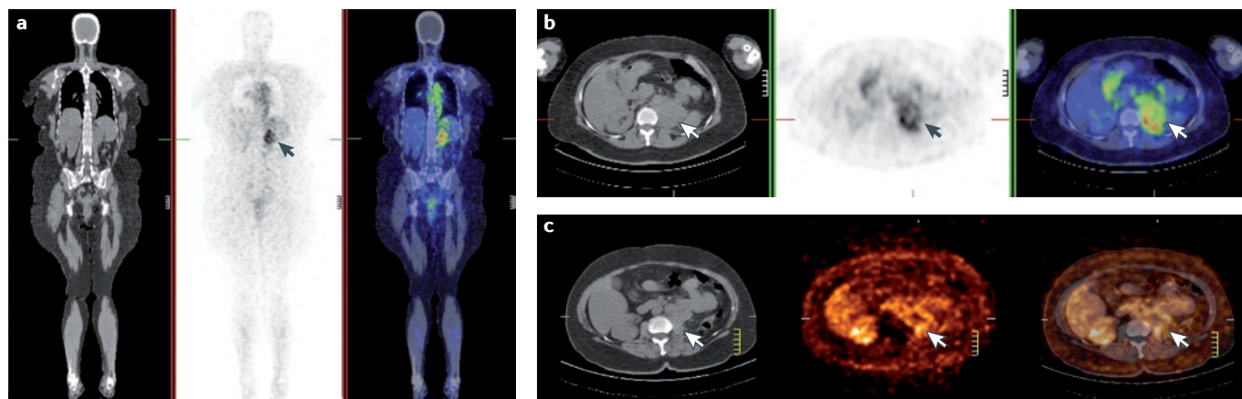
Figure 2 | Biodistribution and pharmacodynamics of an antibody in vivo. a | Whole-body coronal positron emission tomography–computed tomography (PET–CT) images of ^{124}\text{I} -labelled cG250 (carbonic anhydrase IX (CAIX)-specific) monoclonal antibody, obtained 5 days after antibody infusion. The specific uptake of the antibody can be seen in the left renal tumour (arrow), which is expressing CAIX antigen. A quantitative concentration of an antibody in a tumour can be measured using this imaging methodology. Some normal blood pool activity can also be seen, owing to the antibody circulating in blood, but no other tissues show antibody localization. b | Transaxial PET–CT images through the left kidney mass, showing antibody localization in the tumour in detail (arrow). The right-hand panel shows combined (fused) PET–CT images. c | A quantitative tumour blood flow assessment using \text{H}_2\ ^{15}\text{O} PET–CT. Tumour perfusion is readily apparent (arrow) in the left kidney mass. Pharmacodynamic changes in the tumour following treatment can be assessed non-invasively using imaging techniques.
