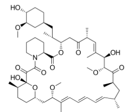
Rapamycin (Sirolimus) C 51 H 79 NO 13 MW: 914.172
